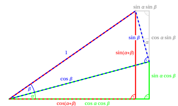
Additionstheoreme
